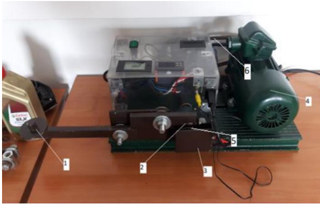
Fig. 1. The Timken test experimental setup: 1 – lever with the load, 2 – sample, 3 – oil bath, 4 – electric motor, 5 – shaft
