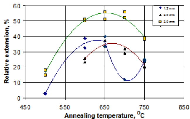
Fig. 2. Effect of annealing temperature on relative extension of the low-carbon steel wire
