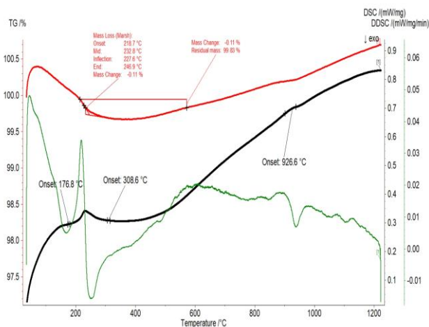
Fig. 3. TG-DSC of the system \text{BaTiO}_3 - \text{BaSnO}_3
