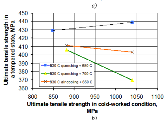
Fig. 13. Effect of initial strength after drawing deformation on the strength obtained after quenching and air cooling (a) and after subsequent tempering (b)
