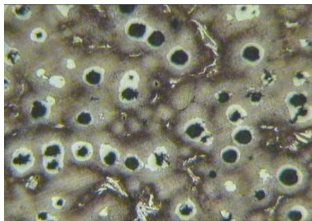
x50- Metal base (perlite) + carbides + spheroidal graphite + ferrite Figure 2.6
