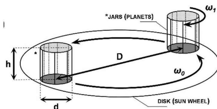
Figure 6. Schematic representation of high-energy ball milling, where the jars revolve around the centre of the sun wheel ( w_0 is the nominal angular velocity) while rotating around their own axis (the corresponding angular velocity, w_1 , being not necessarily equal to w_0 ). In this context, the height ( h ) and diameter ( d ) of the vials are important. Combination of shear, friction, and impacts ( c ) is generated in planetary-type mills.
