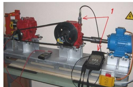
Fig.5. Experimental stand with vibration analyzer: 1 – vibration analysis system C/D-21 [16]
