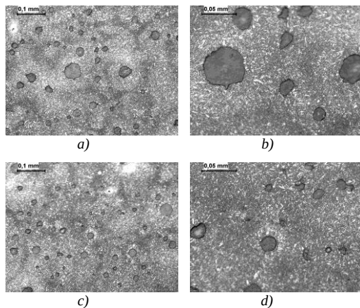
Fig. 6 Microstructure of ductile iron
