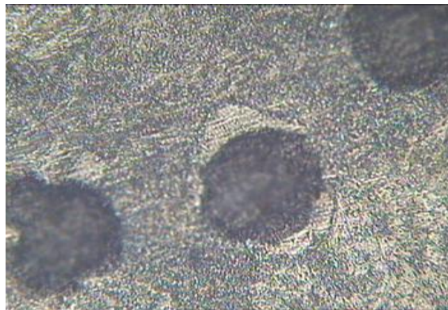
x500- Metal base (perlite) + spheroidal graphite Figure 2.5
