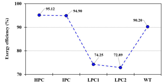
Fig. 4. The exergy efficiency of the whole observed steam turbine and each cylinder
