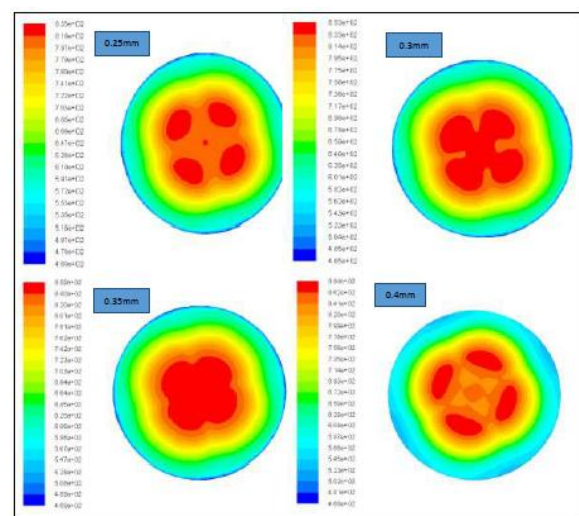
Fig. 7 Pot bottom temperature for 8 mbar fuel pressure.
