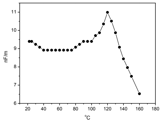
Fig. 5. \epsilon_r of \text{BaTiO}_3 - \text{BaSnO}_3 in ratio (85%:15%) ceramic pellet vs the temperature of the pellet.
