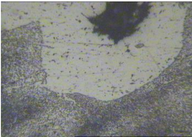
II x200 - Metal base (perlite) + graphite with spheroidal shape + ferrite
