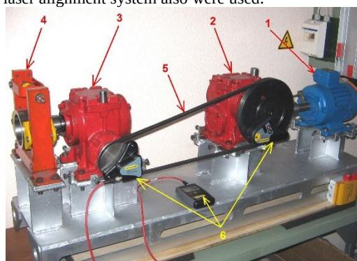
Fig.2. Experimental stand: 1 – electromotor, 2 - worm gearbox Nr.1, 3 - worm gearbox Nr.2, 4 - brake mechanism, 5 - v-belt transmission, 6 – laser alignment system [10]
