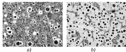
Fig. 4 Microstructure of ductile iron a) test specimen 1.0 NL 400; b) test specimen 2.0 NL 700.
