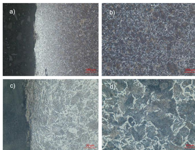
Fig. 6 Microstructure of first forgings a)100x and c)500x near the surface, b)100x and d)500x near the center of the sample, normalized at 860°C for 4.5h and cooled in slow air
