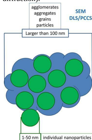
Figure 3. Schematic illustrations showing which techniques report the size of individual nanocrystals or of agglomerates/grains of size larger than 100 nm.
