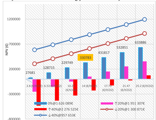
Figure 8: Variation of NPV in function of total investment cost (€) for discount rate 8%, interest rate 5.5% fixed price of electricity 65 €/MWh @ \pm 40\% of sensitivity analysis and sale price of carbon credits (€/tCO 2 ) @ \pm 80\% .
