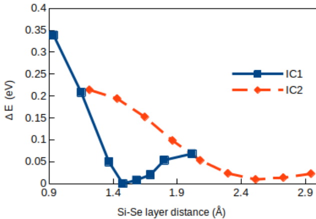
Fig. 2 Total energy relative to its minimum value ( \Delta E = E - E_{\min} ) as a function of the distance d_{\text{Si-Se}} between Si and Se layers for a FeSe monolayer on the Si(001) surface with two possible interface configurations IC1 and IC2.
