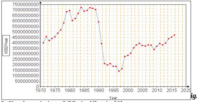
Fig. 2: Yearly variation of CO 2 in Albania [6].
