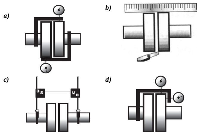
Fig 1. Shaft alignment methods [7]
