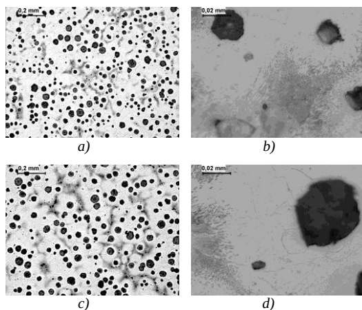
Fig. 5 Microstructure of ductile iron
