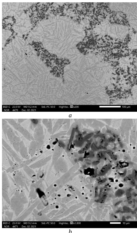
Fig. 5. Back scattered electron image of Ti-Al-C sample: dark carbides, slightly grey \beta -Ti and light particles – possible \text{Ti}_3\text{AlC}
