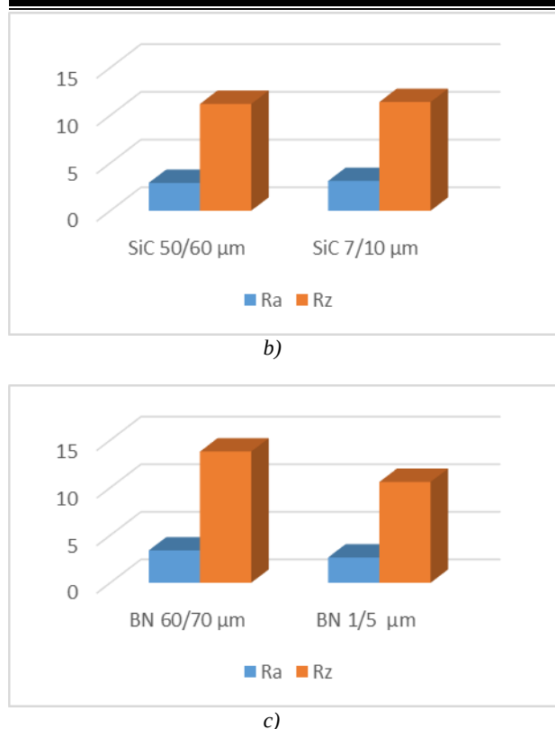
Fig. 2: Change of the roughness parameters R_a and R_z after treatment of the limestone samples with disks with different types and sizes of the particles: a) Diamond particles; b) SiC; c) BN. Values of R_a and R_z before treatment - 3.96 \mu\text{m} and 17.6 \mu\text{m} , respectively.
