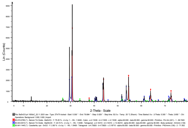
Fig. 2 XRD diagram of synthesized \text{BaTiO}_3 by sol-gel method.
