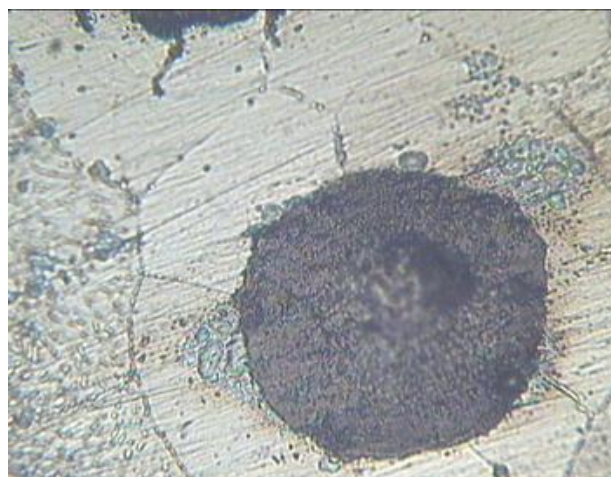
x500- Metal base (perlite) + spheroidal graphite + ferrite Figure 2.7
